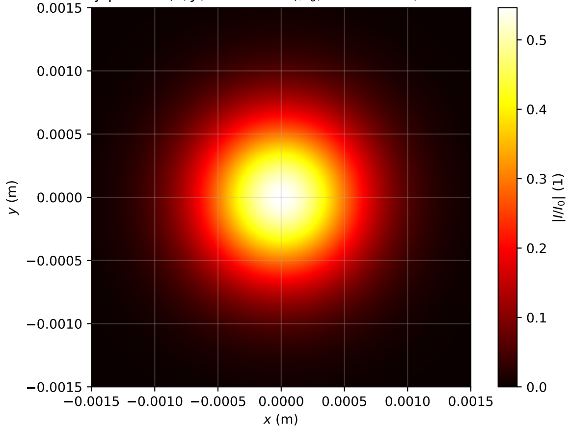
Intensity profile I(x, y, z = 2.707m)/I_0 , Pin=0.4Pcr, artificial time
